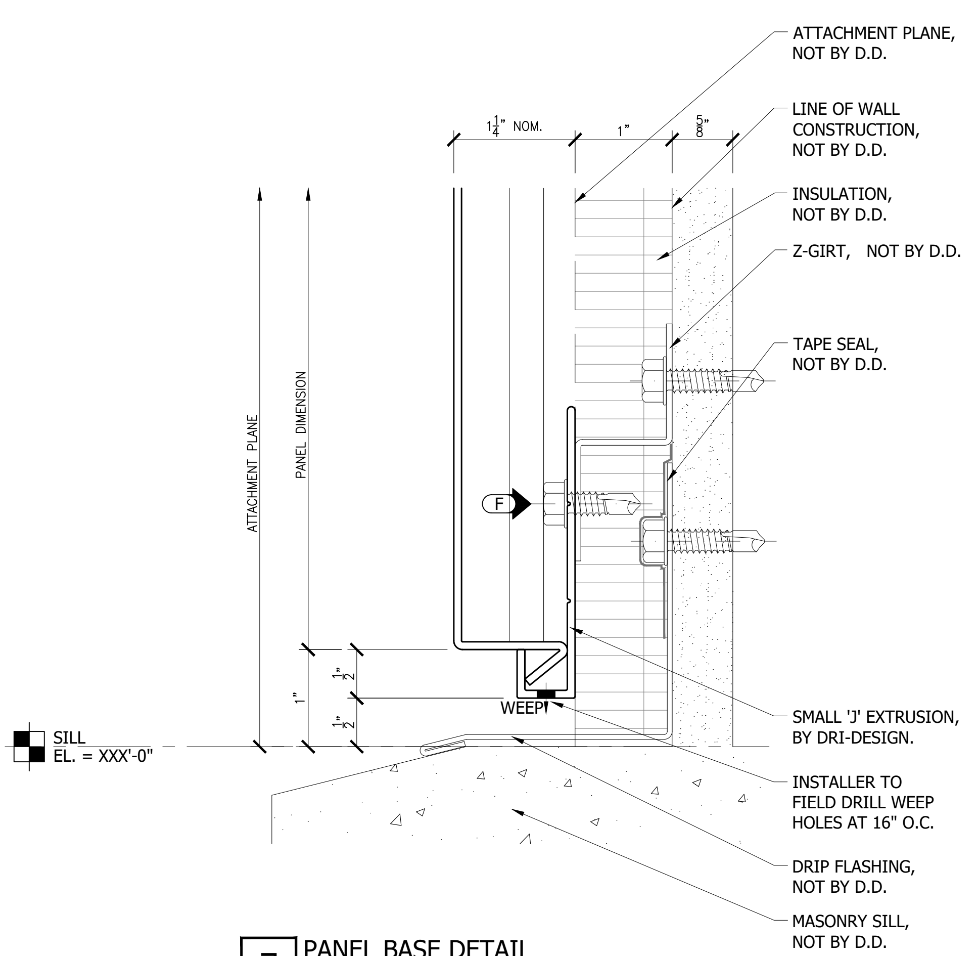
7 PANEL BASE DETAIL REF: --/---
