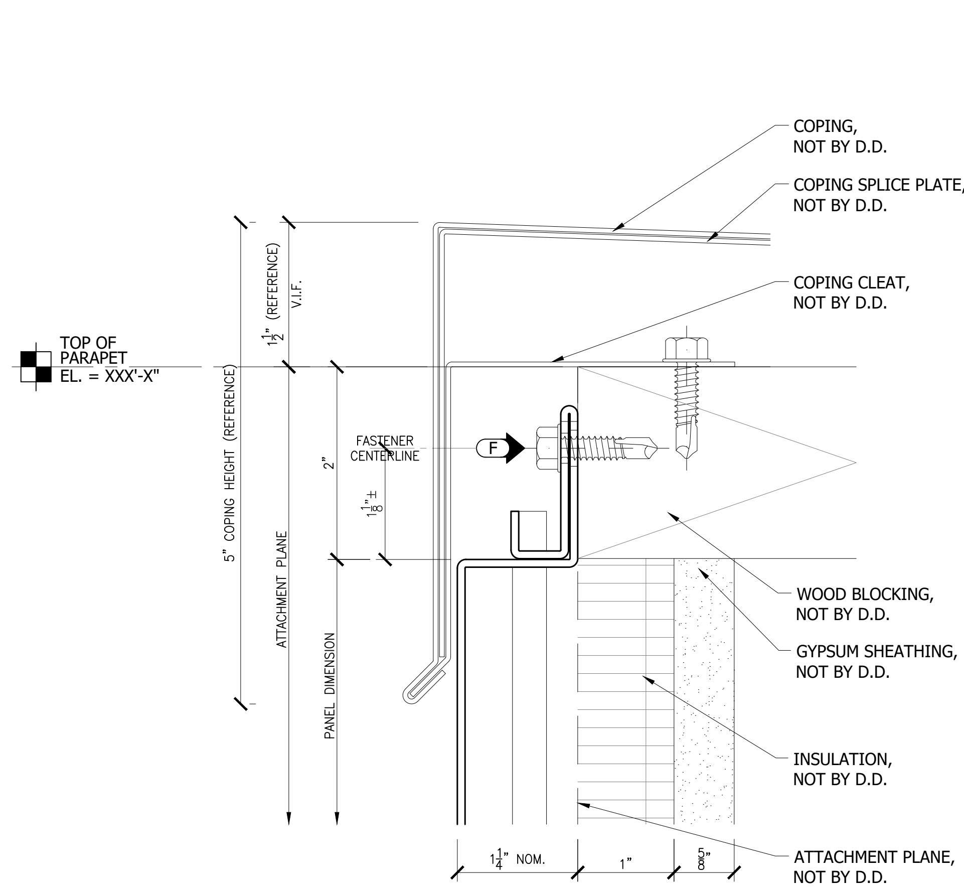
1 OVERLAP COPING/ HEAD DETAIL REF: --/---
