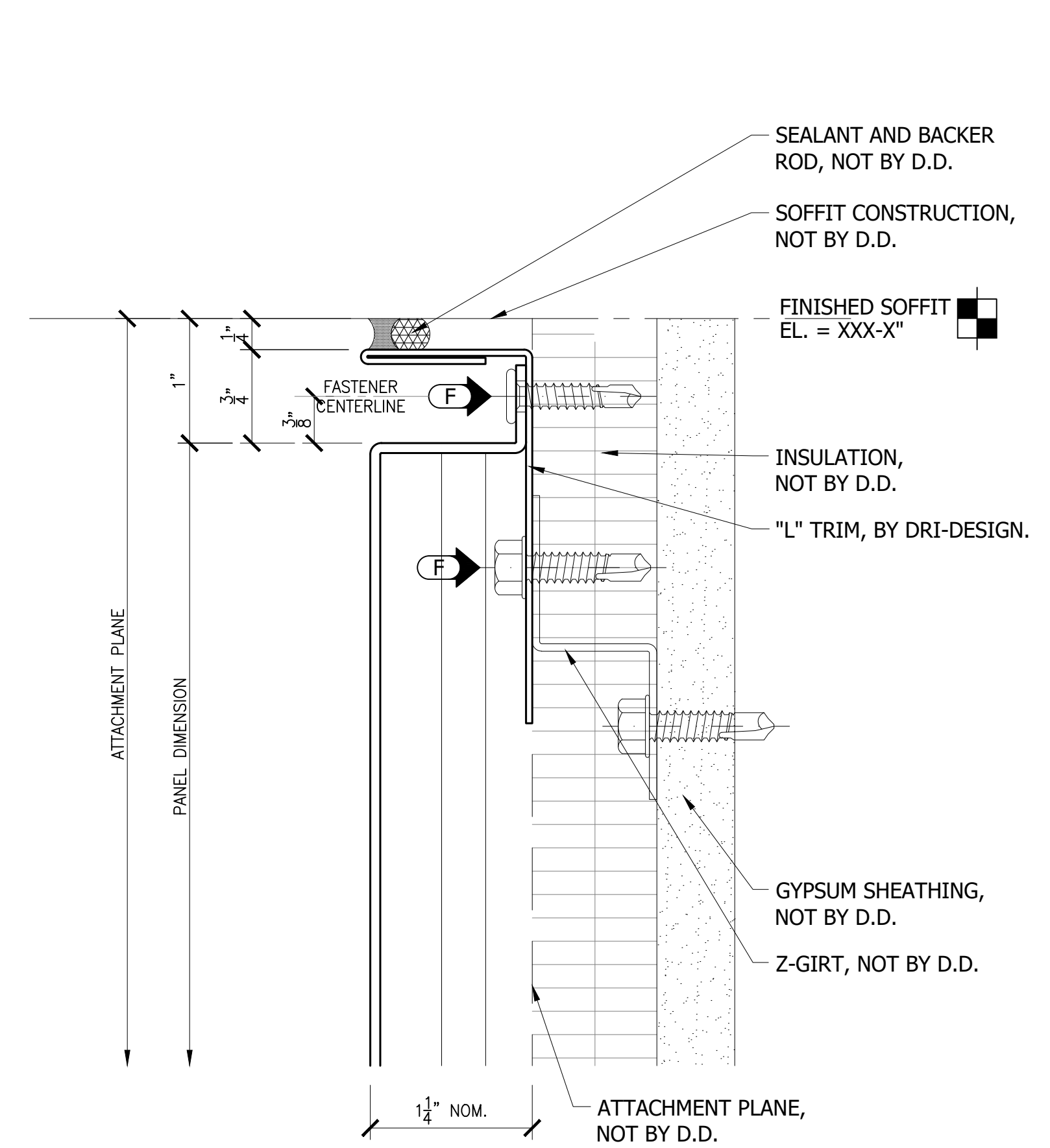
3 PANEL HEAD DETAIL AT SOFFIT REF: --/---
