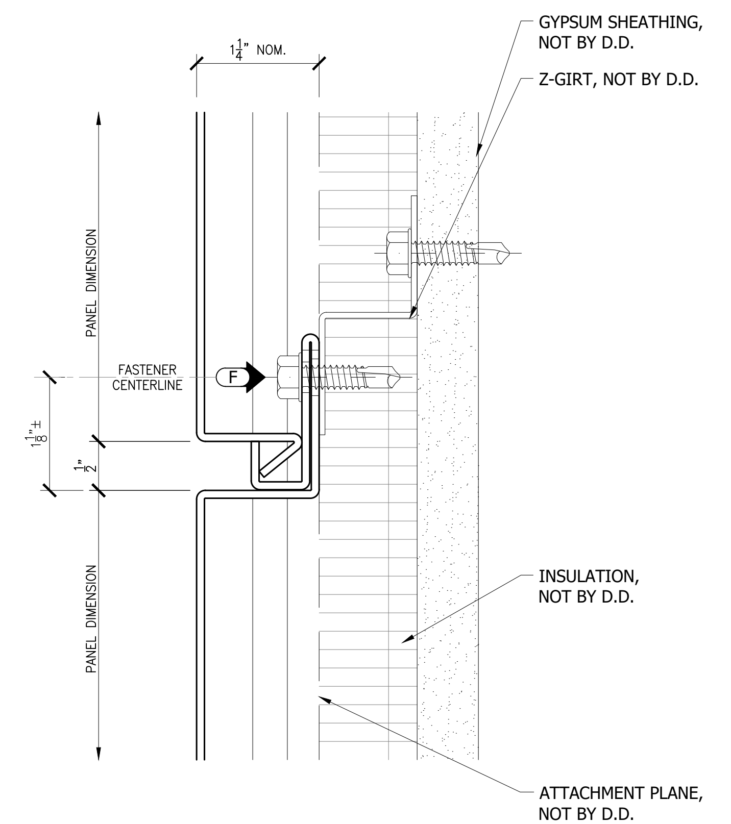
6 1/2" HORIZONTAL JOINT DETAIL REF: --/---
