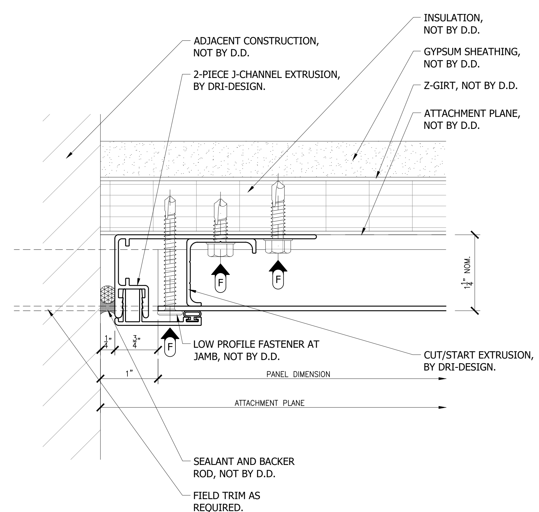
26 CUT-TO-FIT DESIGN JAMB TERMINATION DETAIL REF: --/--
