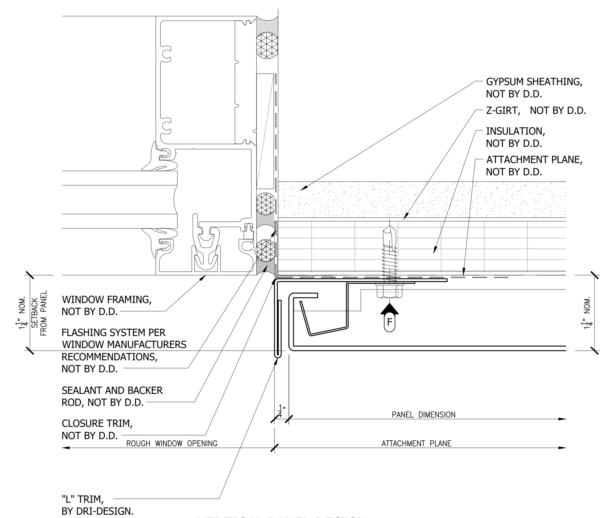
21 VERTICAL PANEL DESIGN JAMB TERMINATION DETAIL AT WINDOW REF: --/---
