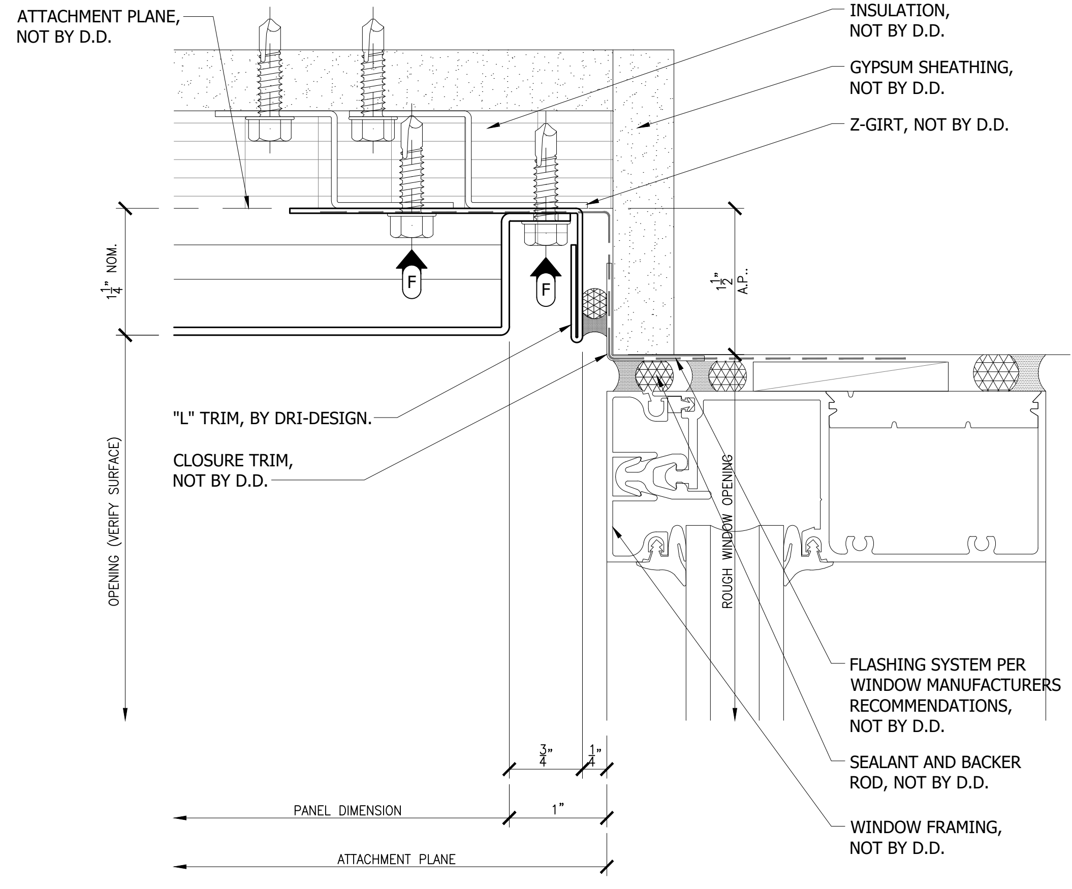
20 JAMB TERMINATION DETAIL AT WINDOW REF: --/---
