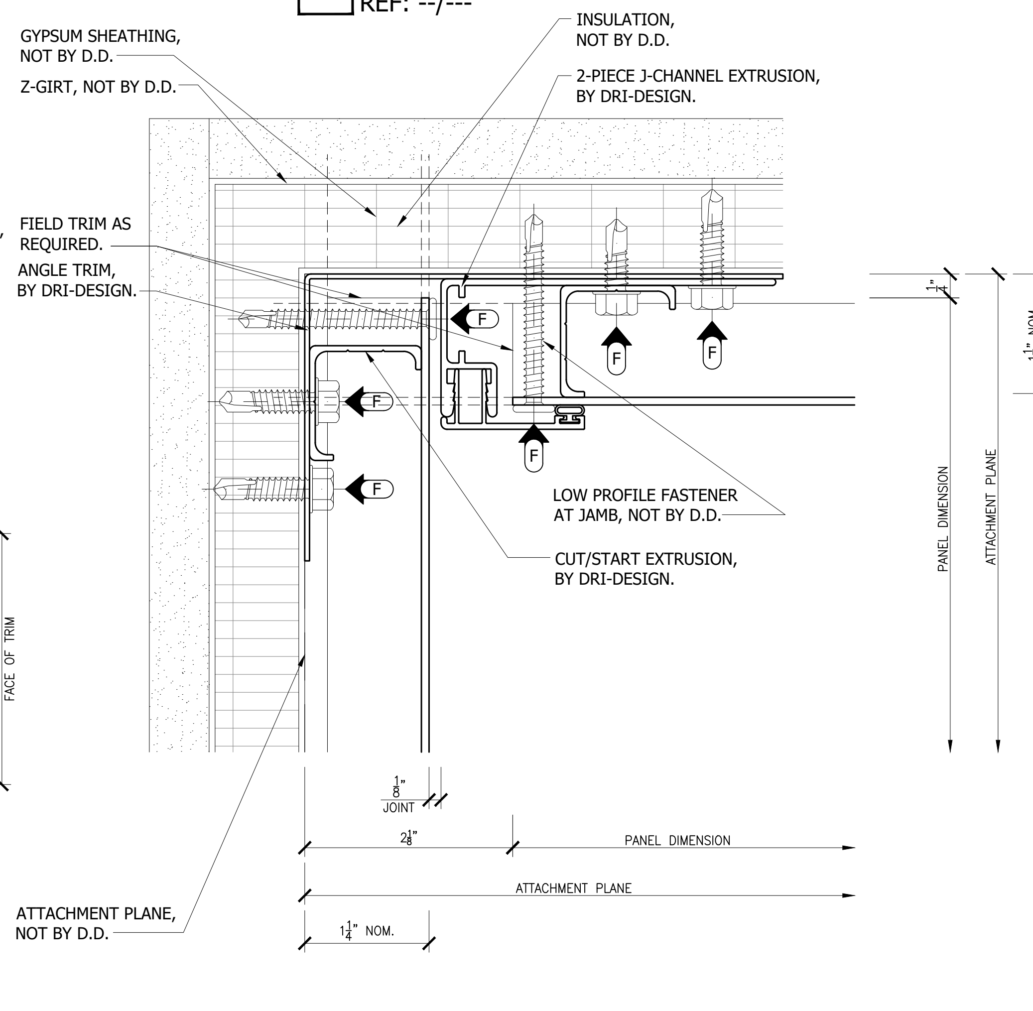
29 CUT-TO-FIT DESIGN 90° INSIDE CORNER DETAIL REF: --/--
