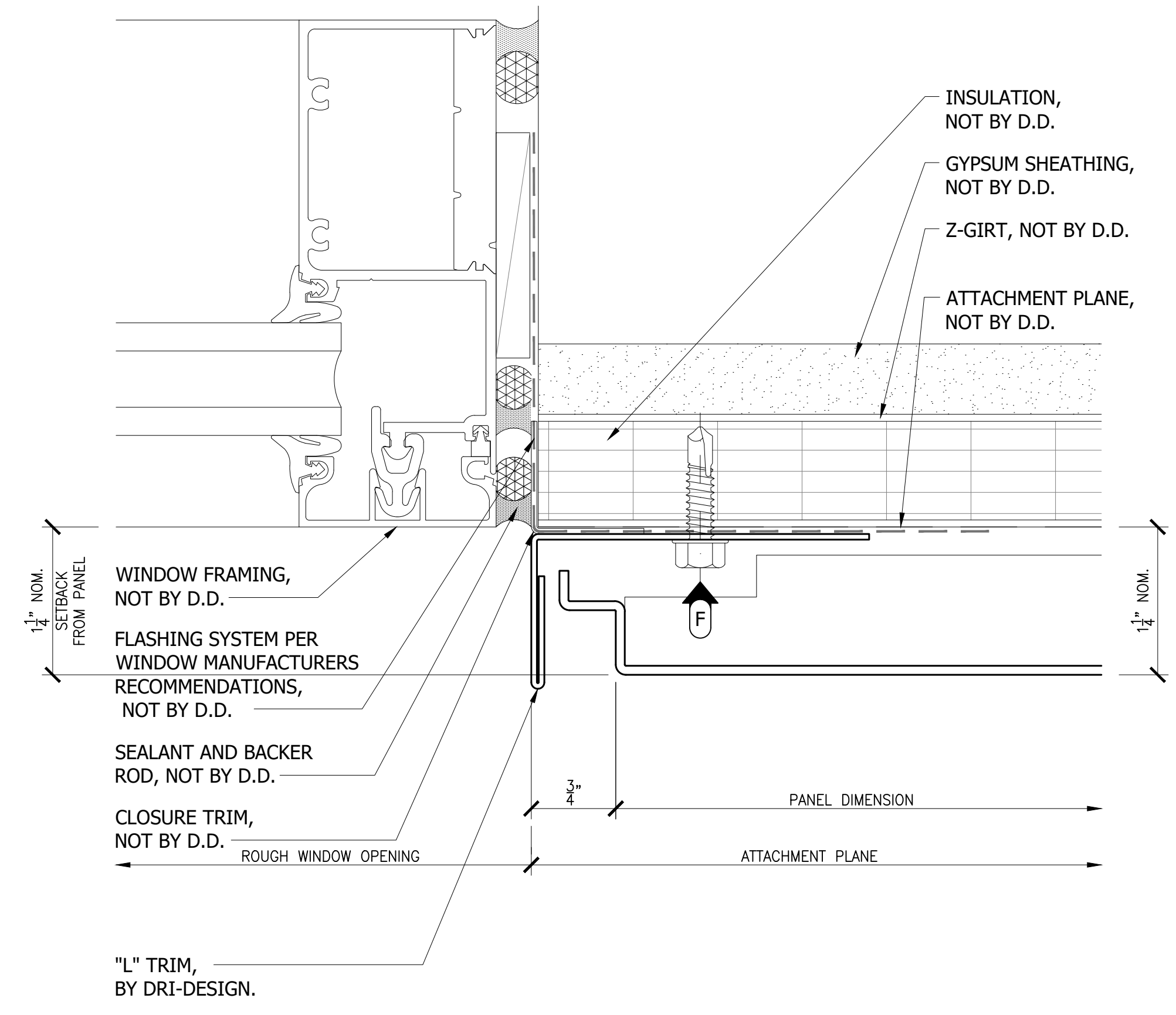
20 JAMB TERMINATION DETAIL AT WINDOW REF: --/---
