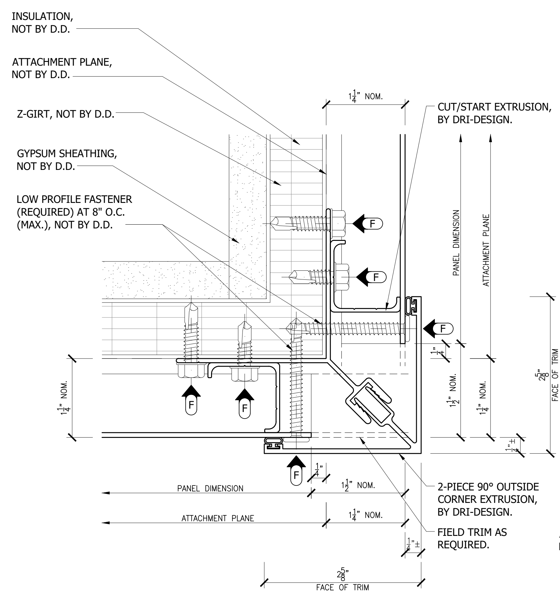
28 CUT-TO-FIT DESIGN 90° OUTSIDE CORNER DETAIL REF: --/--
