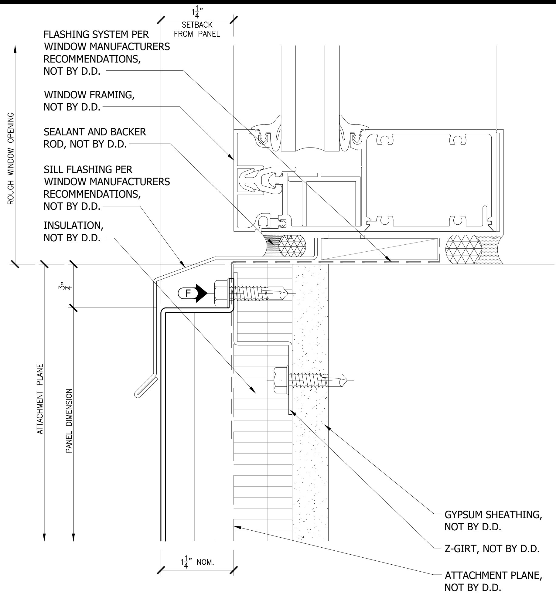
19 PANEL HEAD/WINDOW SILL DETAIL REF: --/---
