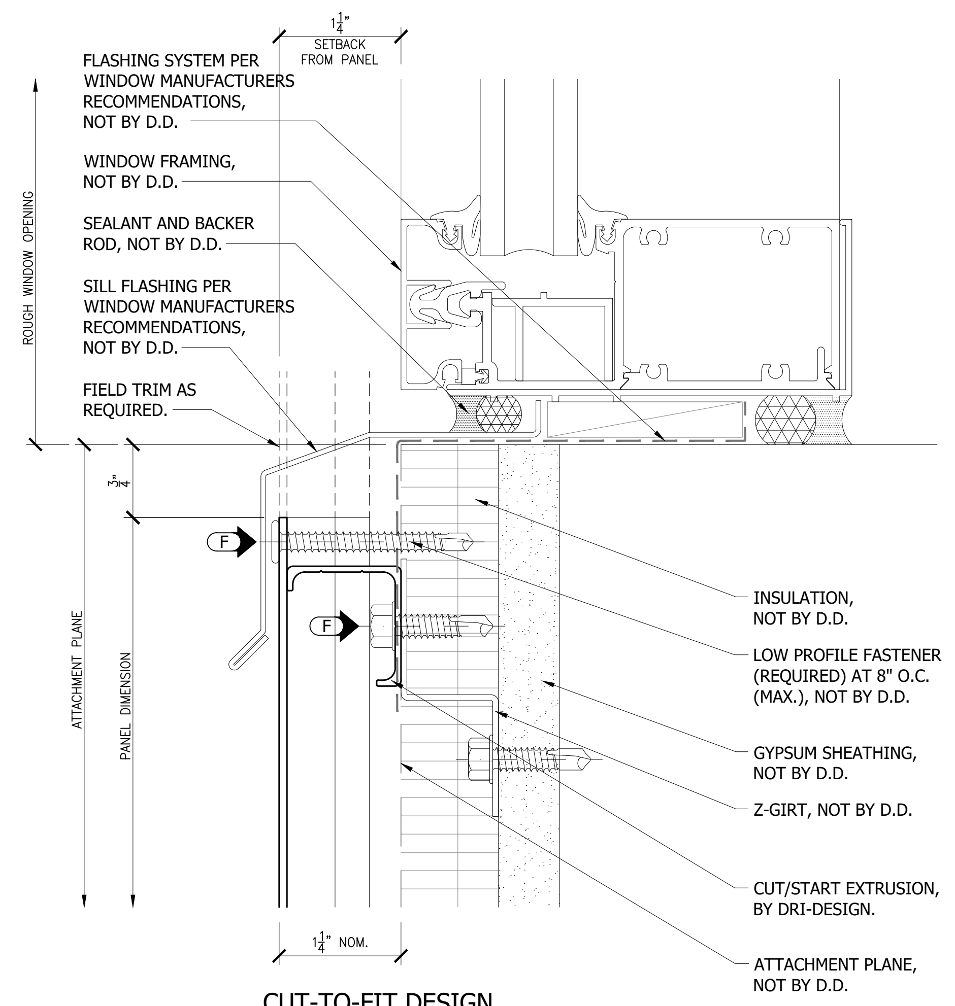
35 CUT-TO-FIT DESIGN PANEL HEAD/ WINDOW SILL DETAIL REF: --/---
