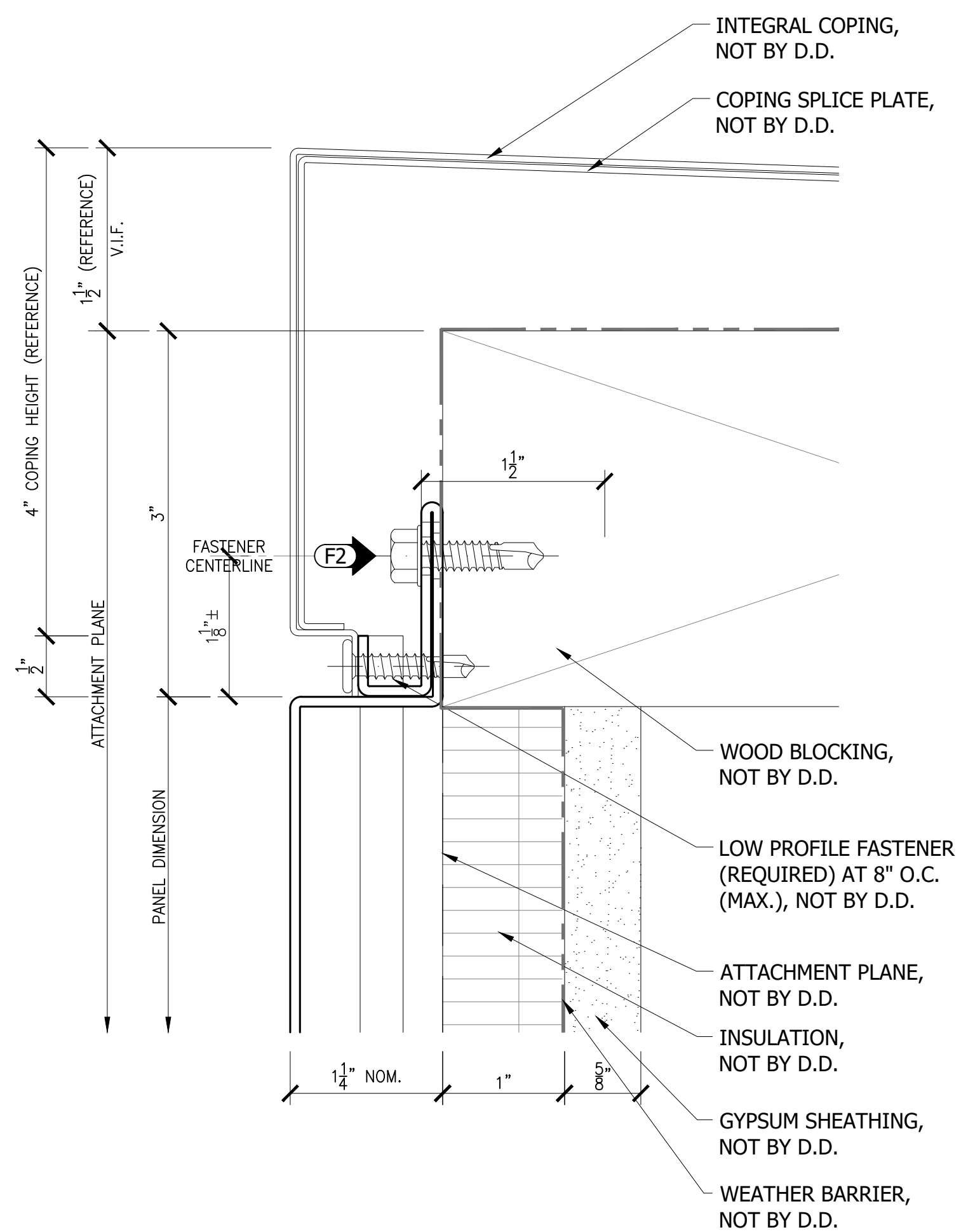
2 INTEGRAL COPING/ HEAD DETAIL REF: --/---
